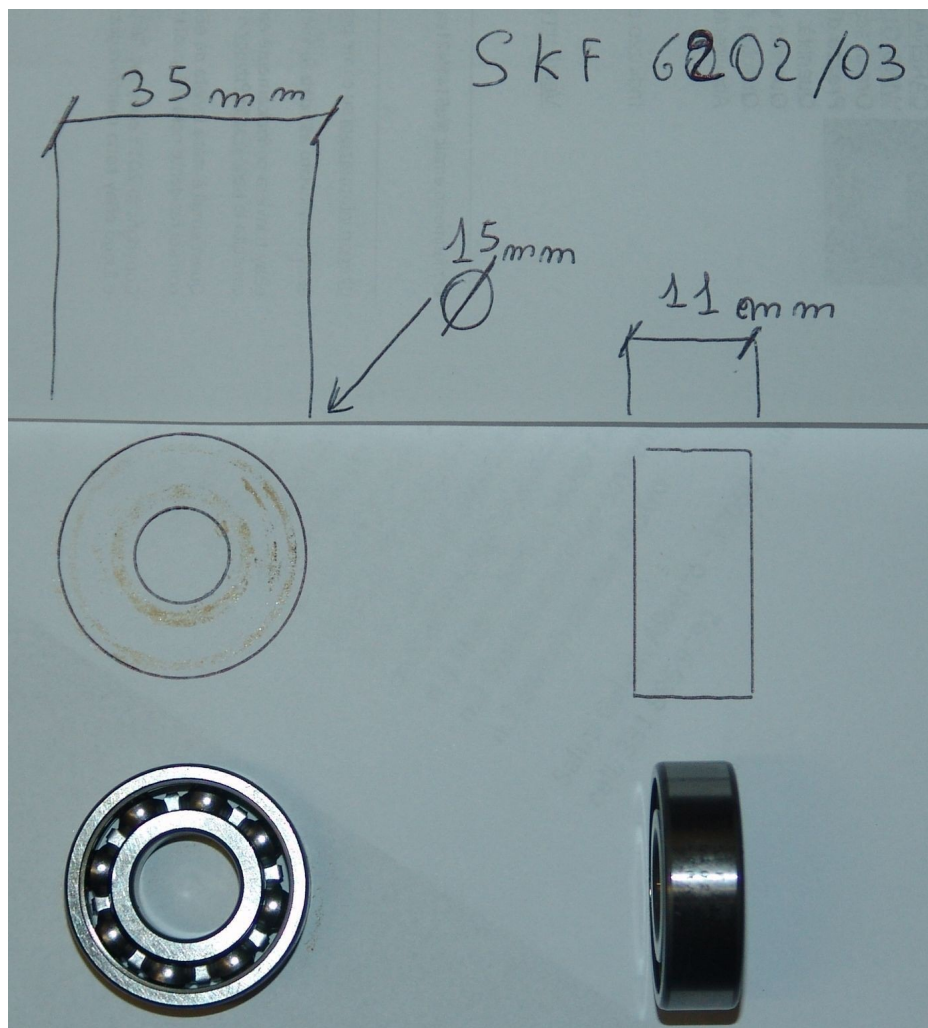
CUSCINETTO BEARING 15 X 35 X 11
